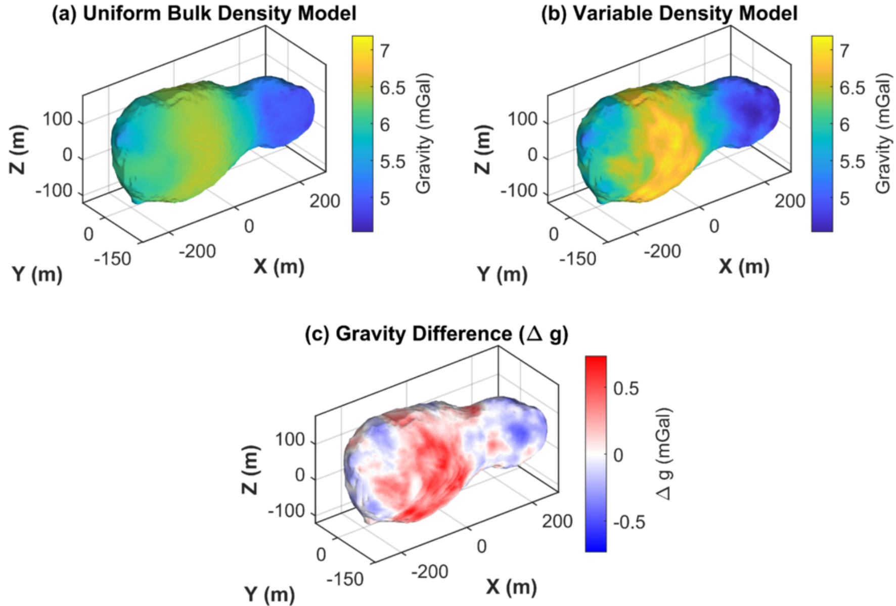
Figure 6. from William Hickmott et al 2026 Planet. Sci. J. 7 doi:10.3847/PSJ/aea569 https://dx.doi.org/10.3847/PSJ/aea569 © 2026. The Author(s). Published by the American Astronomical Society.
