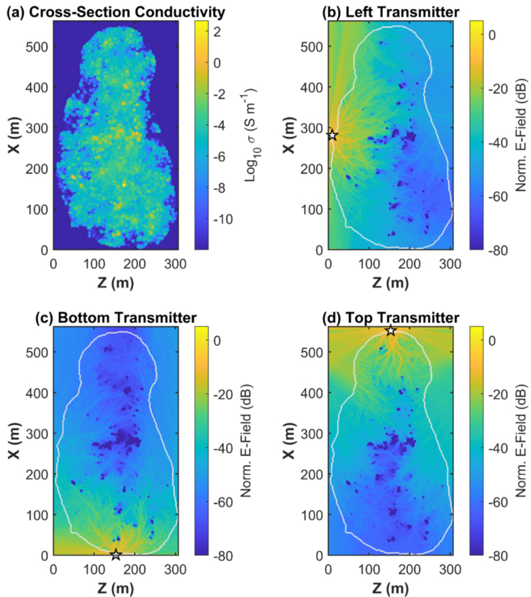
Figure 5. from William Hickmott et al 2026 Planet. Sci. J. 7 doi:10.3847/PSJ/aea569 https://dx.doi.org/10.3847/PSJ/aea569 © 2026. The Author(s). Published by the American Astronomical Society.
