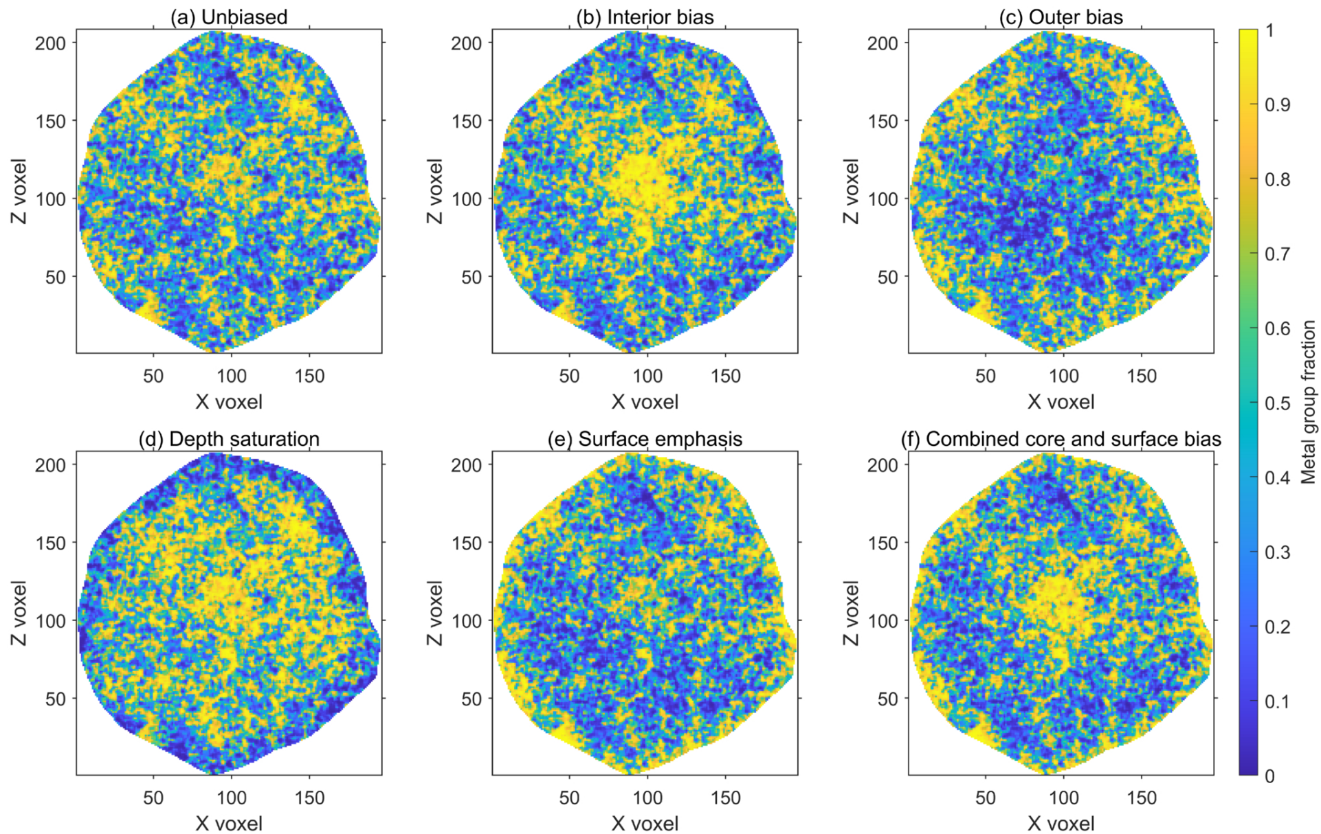
Figure 3. from William Hickmott et al 2026 Planet. Sci. J. 7 doi:10.3847/PSJ/aea569 https://dx.doi.org/10.3847/PSJ/aea569 © 2026. The Author(s). Published by the American Astronomical Society.
