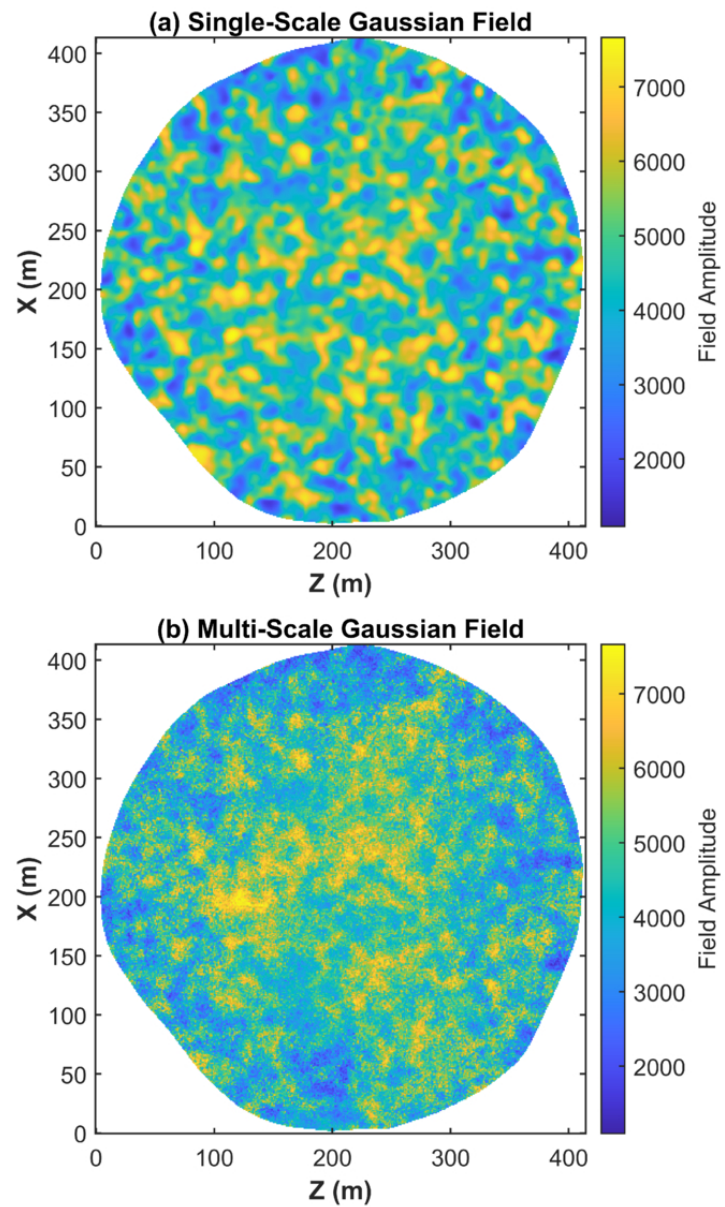
Figure 2. from William Hickmott et al 2026 Planet. Sci. J. 7 doi:10.3847/PSJ/aea569 https://dx.doi.org/10.3847/PSJ/aea569 © 2026. The Author(s). Published by the American Astronomical Society.
