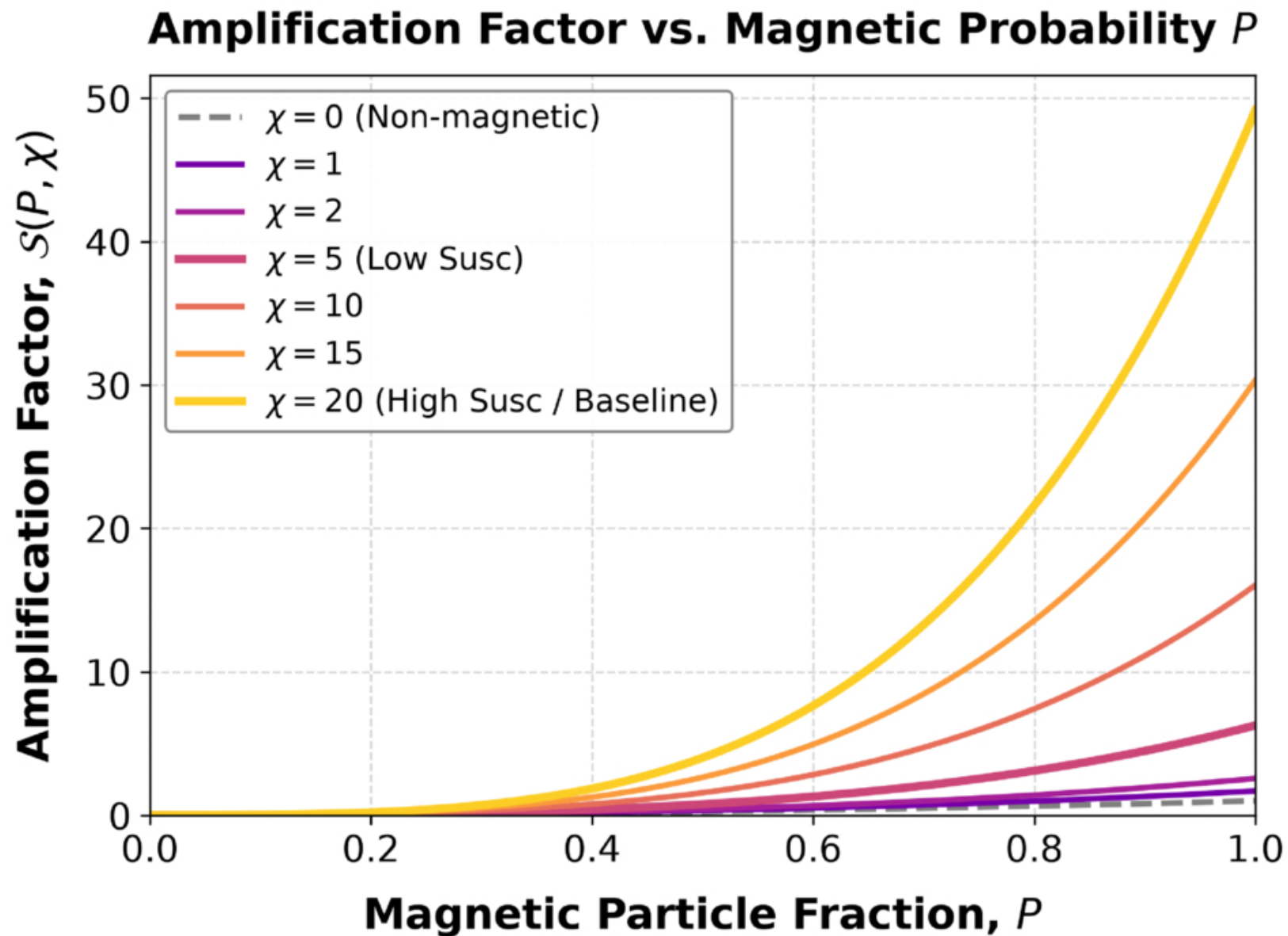
Figure 8. from Anmol Sikka and Christine M. Hartzell 2026 Planet. Sci. J. 7 doi:10.3847/PSJ/aea4b0 https://dx.doi.org/10.3847/PSJ/aea4b0 © 2026. The Author(s). Published by the American Astronomical Society.
