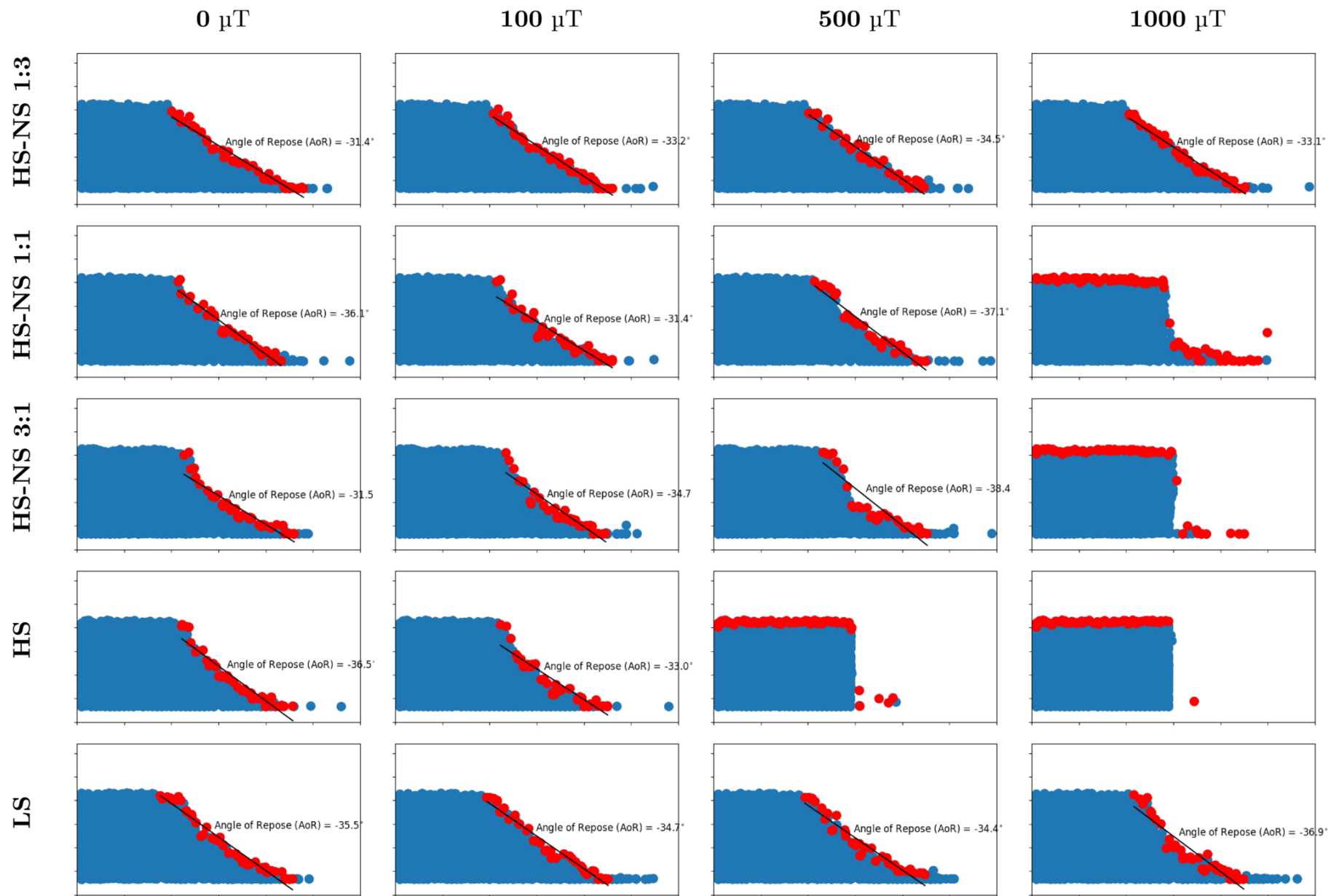
Figure 4. from Anmol Sikka and Christine M. Hartzell 2026 Planet. Sci. J. 7 doi:10.3847/PSJ/aea4b0 https://dx.doi.org/10.3847/PSJ/aea4b0 © 2026. The Author(s). Published by the American Astronomical Society.
