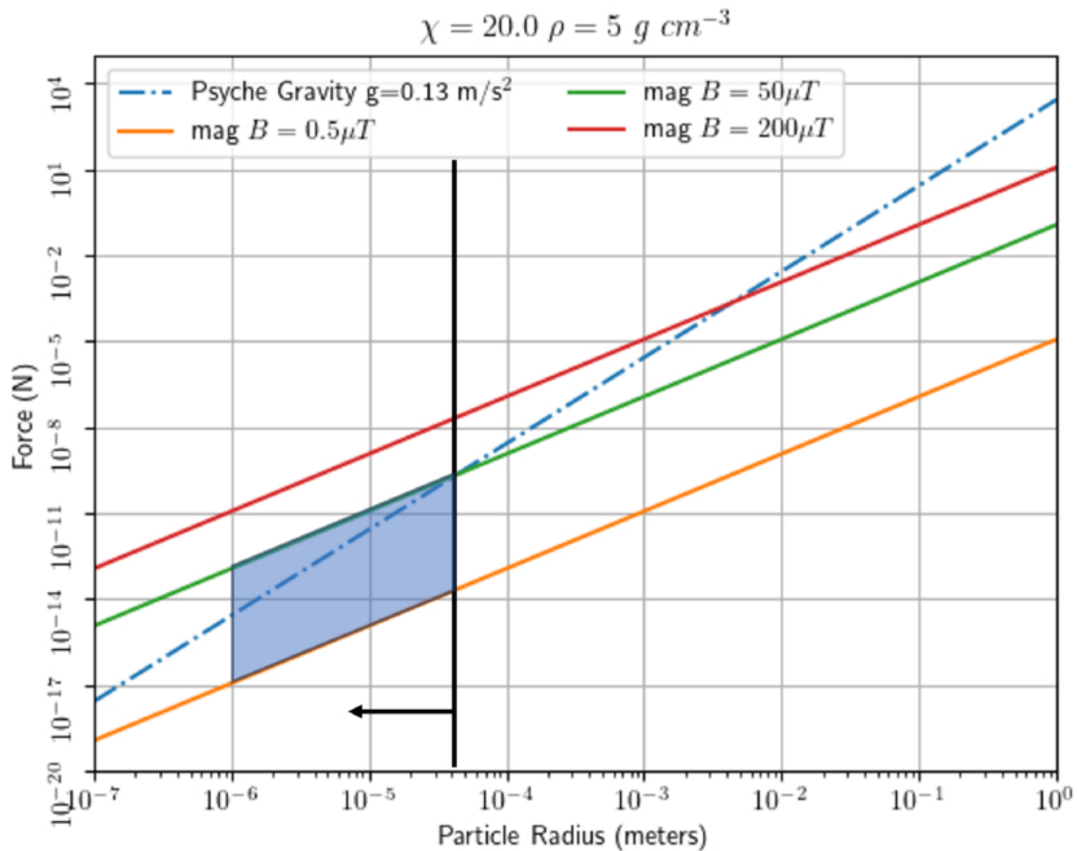
Figure 2. from Anmol Sikka and Christine M. Hartzell 2026 Planet. Sci. J. 7 doi:10.3847/PSJ/aea4b0 https://dx.doi.org/10.3847/PSJ/aea4b0 © 2026. The Author(s). Published by the American Astronomical Society.
