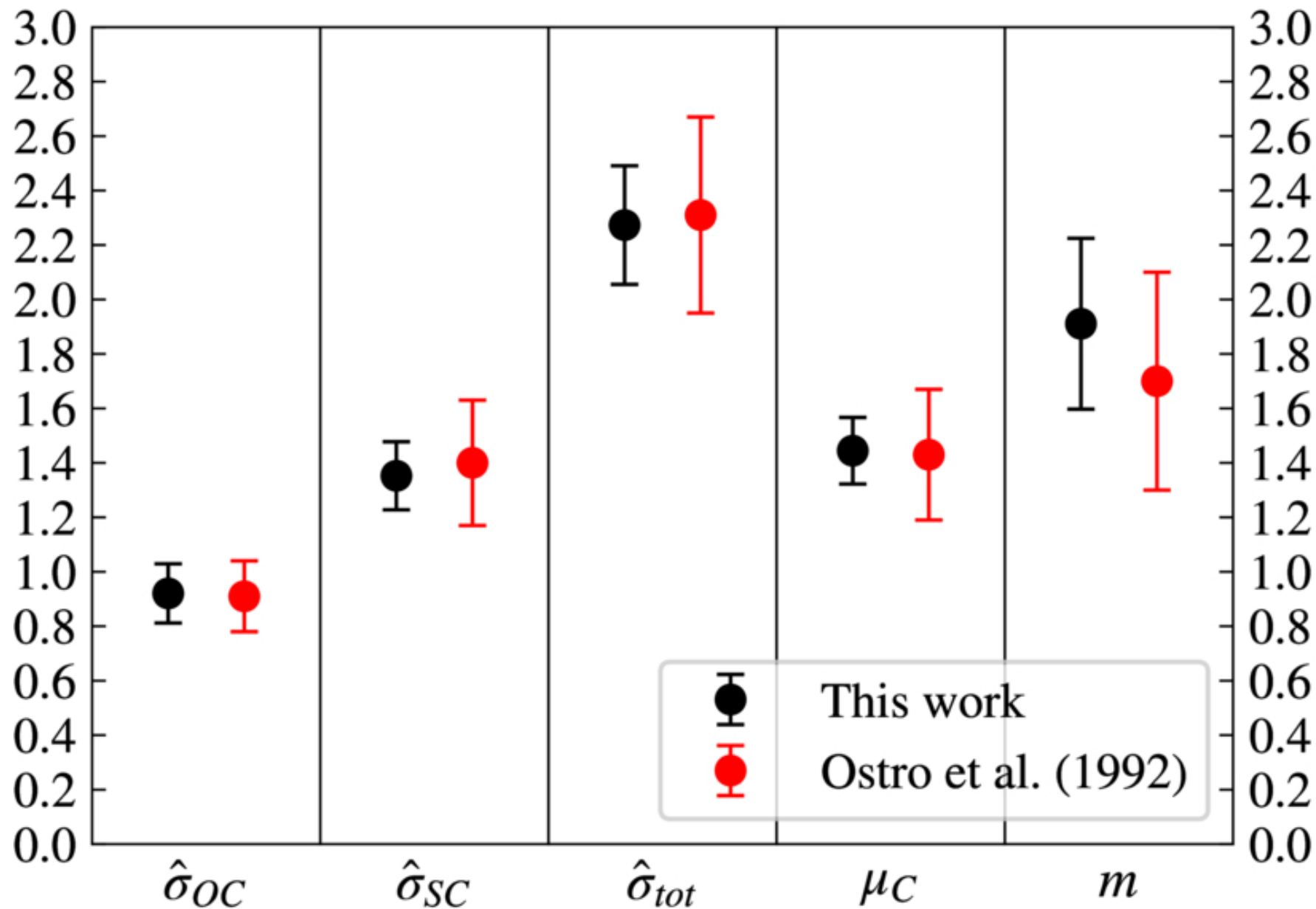
Figure 9. from Tunhui Xie et al 2026 Planet. Sci. J. 7 doi:10.3847/PSJ/aea416 https://dx.doi.org/10.3847/PSJ/aea416 © 2026. The Author(s). Published by the American Astronomical Society.
