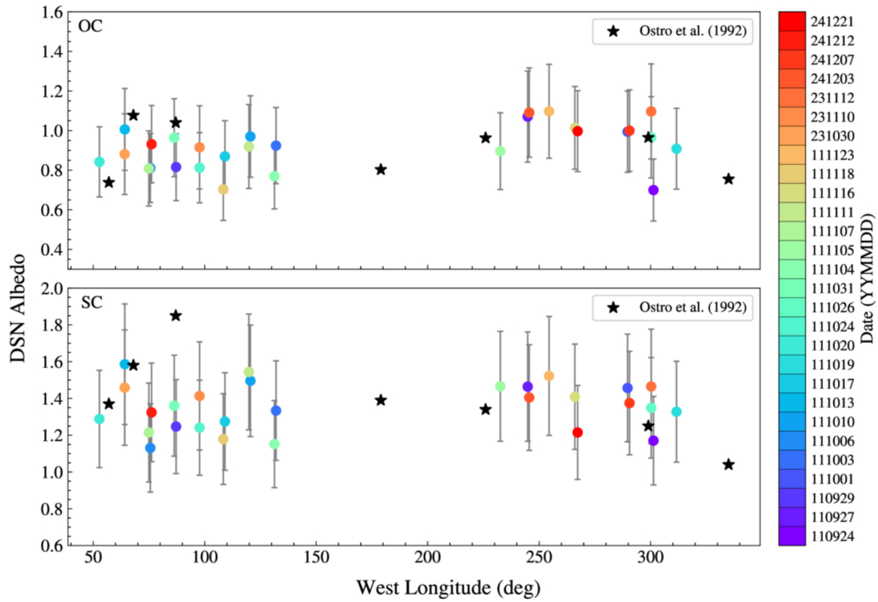
Figure 8. from Tunhui Xie et al 2026 Planet. Sci. J. 7 doi:10.3847/PSJ/aea416 https://dx.doi.org/10.3847/PSJ/aea416 © 2026. The Author(s). Published by the American Astronomical Society.
