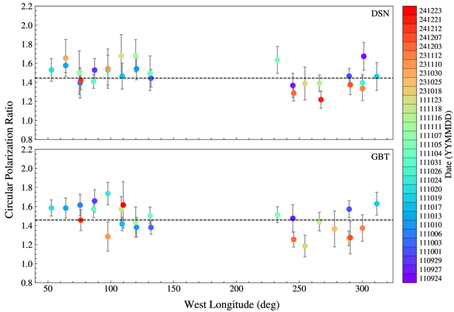
Figure 7. from Tunhui Xie et al 2026 Planet. Sci. J. 7 doi:10.3847/PSJ/aea416 https://dx.doi.org/10.3847/PSJ/aea416 © 2026. The Author(s). Published by the American Astronomical Society.
