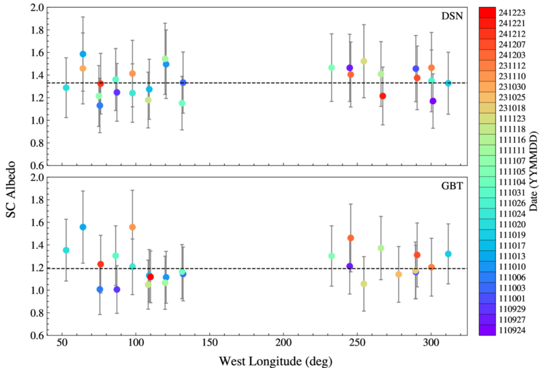
Figure 6. from Tunhui Xie et al 2026 Planet. Sci. J. 7 doi:10.3847/PSJ/aea416 https://dx.doi.org/10.3847/PSJ/aea416 © 2026. The Author(s). Published by the American Astronomical Society.
