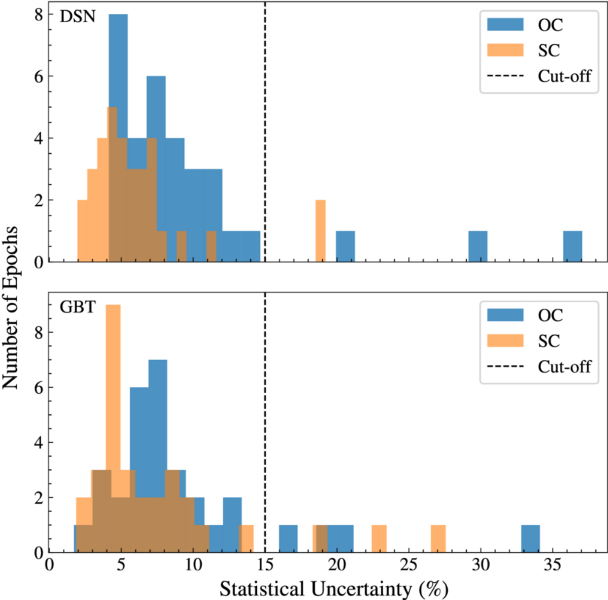
Figure 4. from Tunhui Xie et al 2026 Planet. Sci. J. 7 doi:10.3847/PSJ/aea416 https://dx.doi.org/10.3847/PSJ/aea416 © 2026. The Author(s). Published by the American Astronomical Society.
