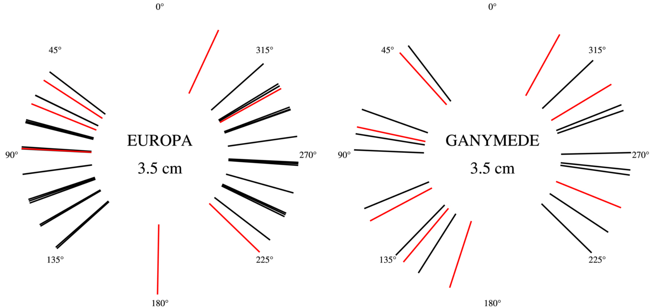
Figure 1. from Tunhui Xie et al 2026 Planet. Sci. J. 7 doi:10.3847/PSJ/aea416 https://dx.doi.org/10.3847/PSJ/aea416 © 2026. The Author(s). Published by the American Astronomical Society.
