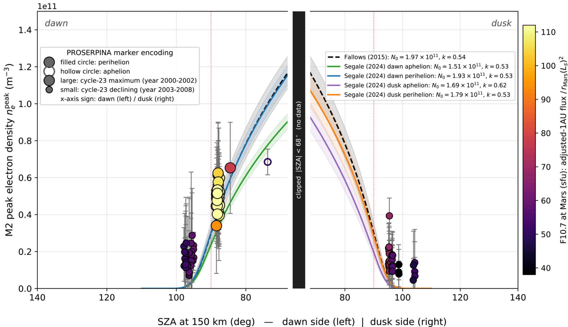
M2 peak electron density vs SZA — PROSERPINA vs Fallows (2015) and Segale (2024) 100 profiles
