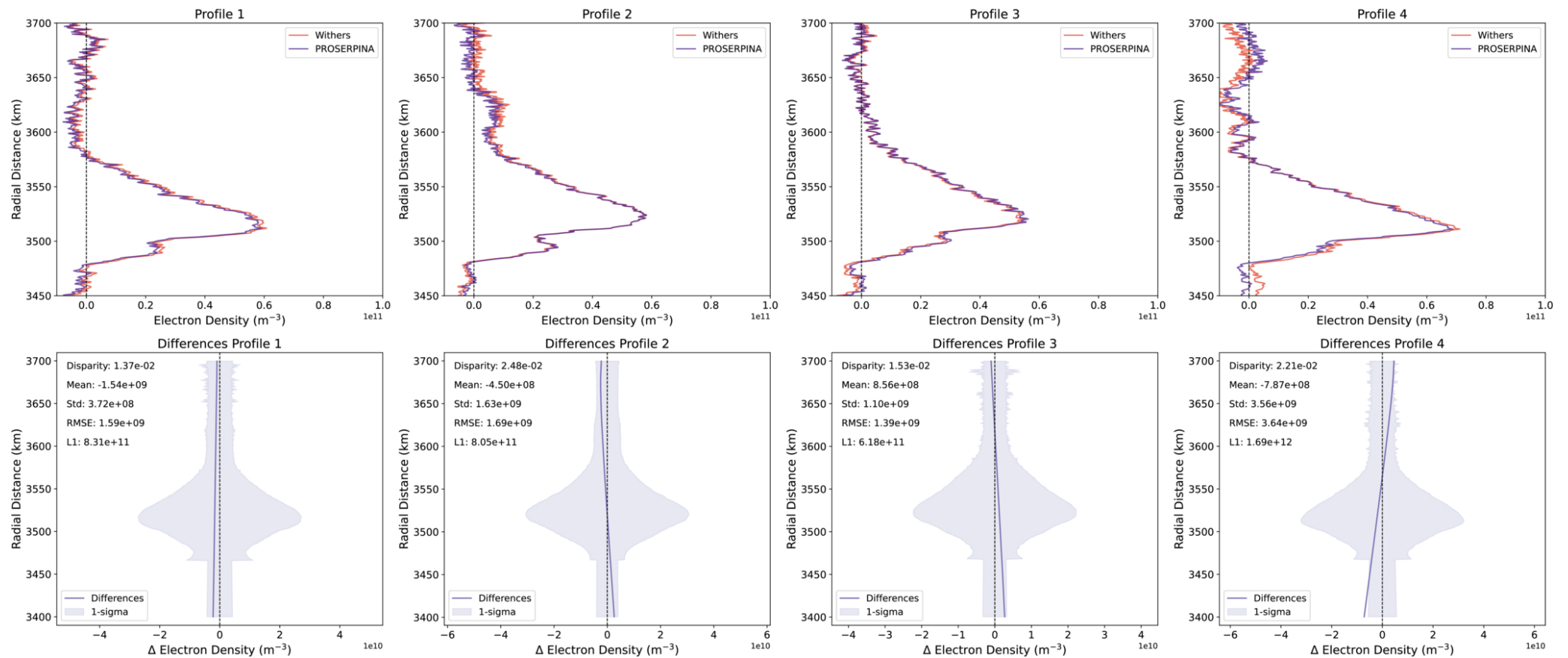
Figure 5. from Marianna Felici et al 2026 Planet. Sci. J. 7 doi:10.3847/PSJ/aea408 https://dx.doi.org/10.3847/PSJ/aea408 © 2026. The Author(s). Published by the American Astronomical Society.
