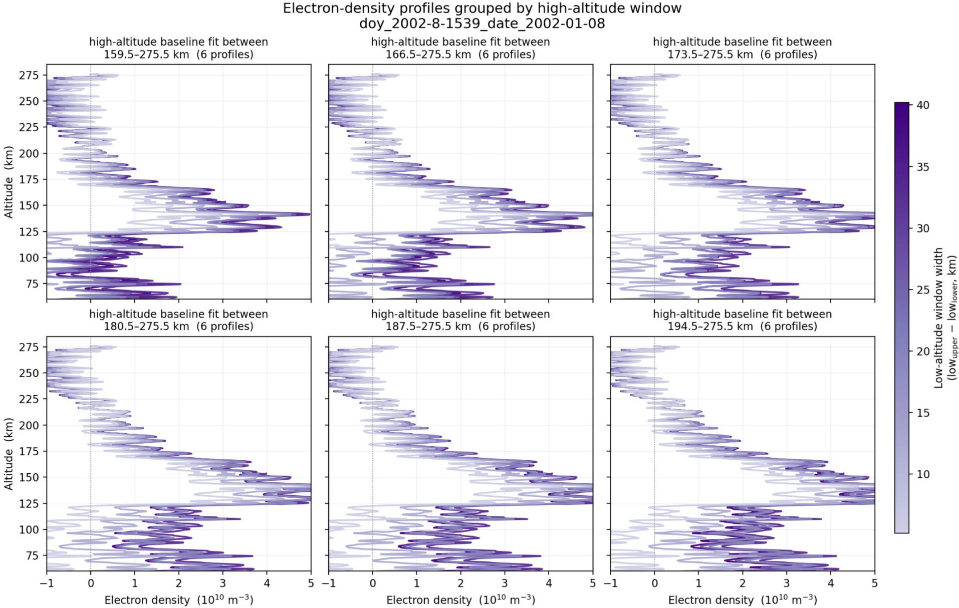
Figure 3. from Marianna Felici et al 2026 Planet. Sci. J. 7 doi:10.3847/PSJ/aea408 https://dx.doi.org/10.3847/PSJ/aea408 © 2026. The Author(s). Published by the American Astronomical Society.
