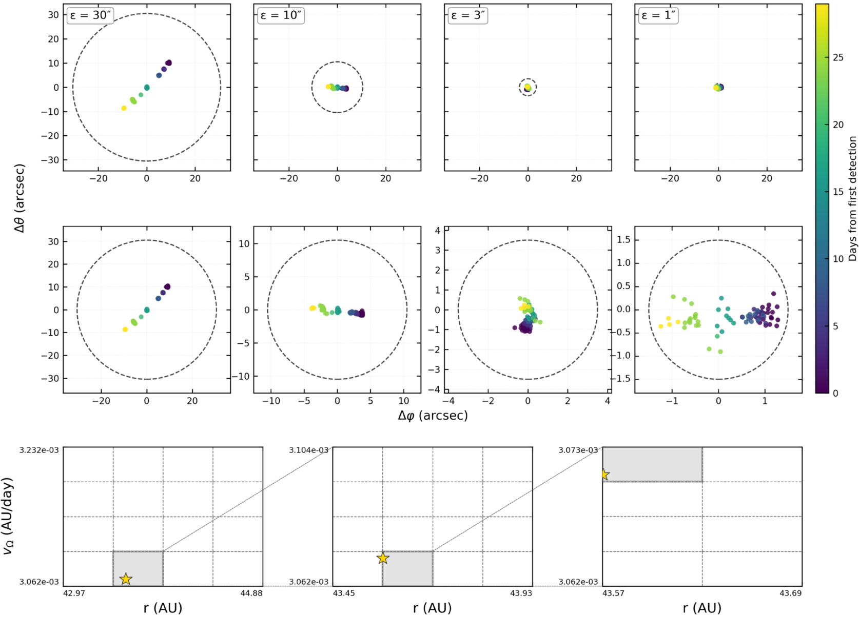
Figure 7. from Thomas R. Ruch et al 2026 Planet. Sci. J. 7 doi:10.3847/PSJ/aea3f4 https://dx.doi.org/10.3847/PSJ/aea3f4 © 2026. The Author(s). Published by the American Astronomical Society.
