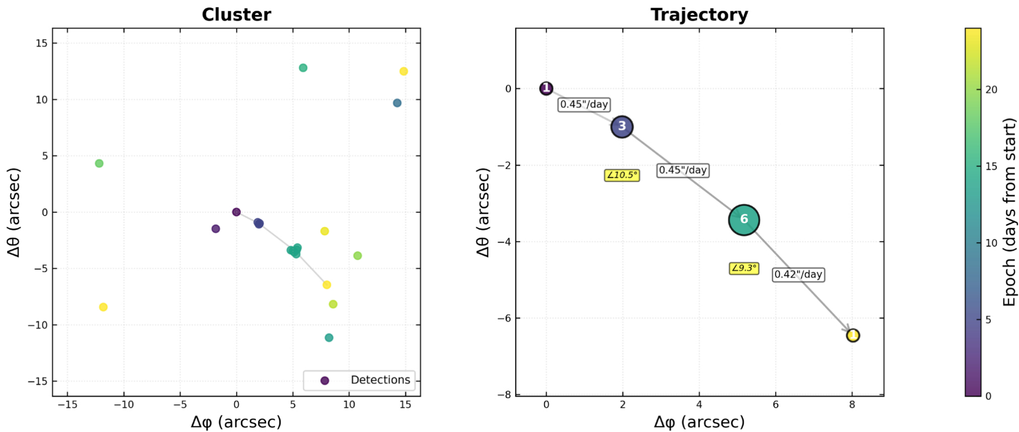
Figure 5. from Thomas R. Ruch et al 2026 Planet. Sci. J. 7 doi:10.3847/PSJ/aea3f4 https://dx.doi.org/10.3847/PSJ/aea3f4 © 2026. The Author(s). Published by the American Astronomical Society.
