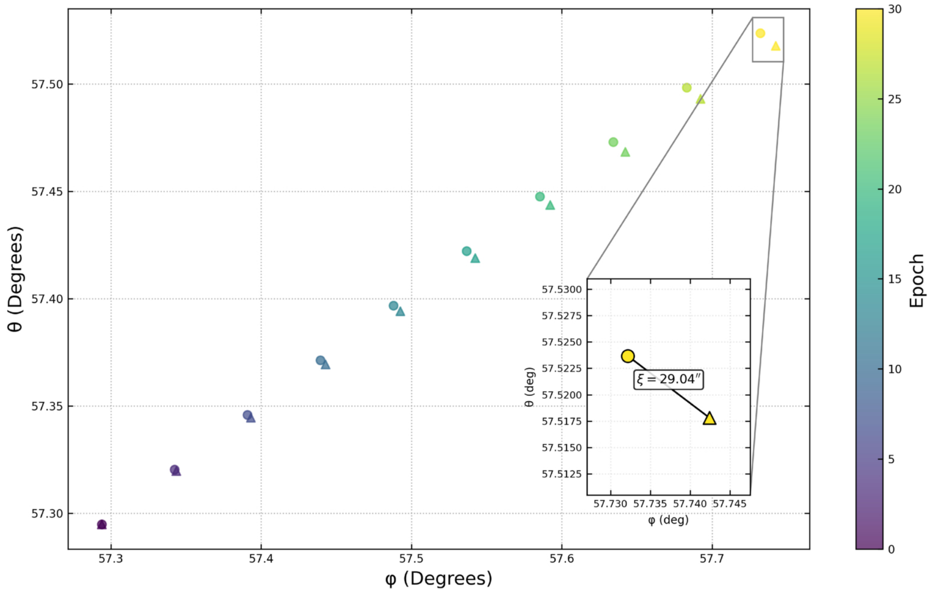
Figure 2. from Thomas R. Ruch et al 2026 Planet. Sci. J. 7 doi:10.3847/PSJ/aea3f4 https://dx.doi.org/10.3847/PSJ/aea3f4 © 2026. The Author(s). Published by the American Astronomical Society.
