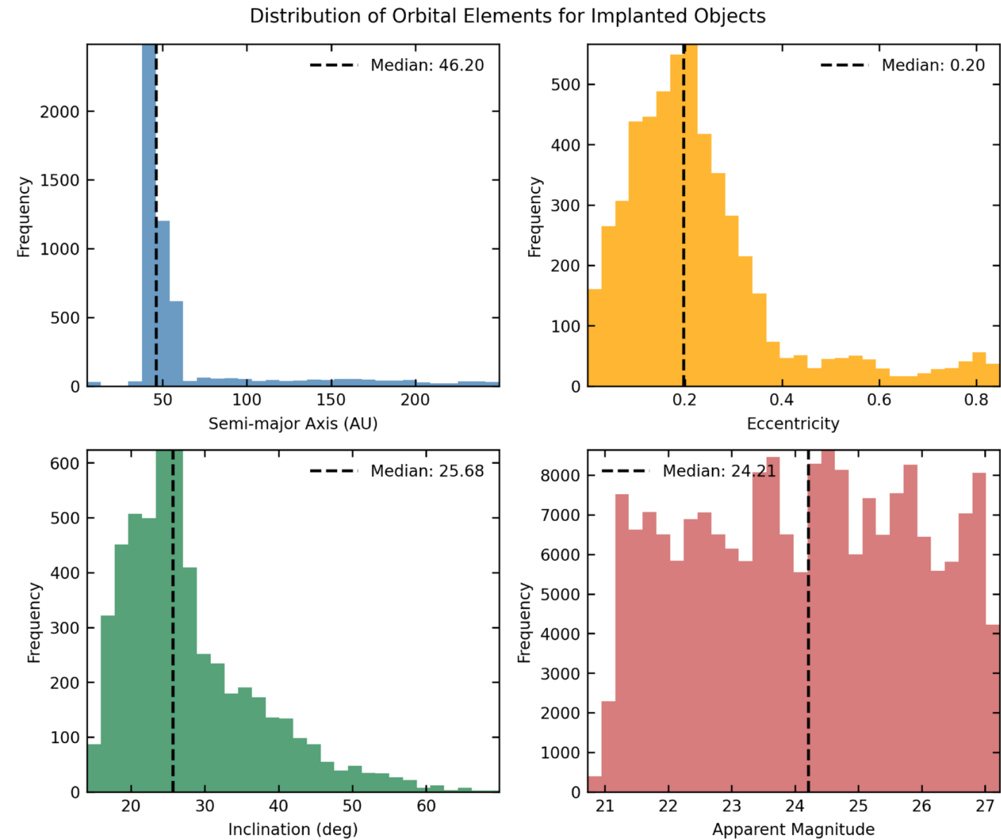
Figure B1. from Thomas R. Ruch et al 2026 Planet. Sci. J. 7 doi:10.3847/PSJ/aea3f4 https://dx.doi.org/10.3847/PSJ/aea3f4 © 2026. The Author(s). Published by the American Astronomical Society.
