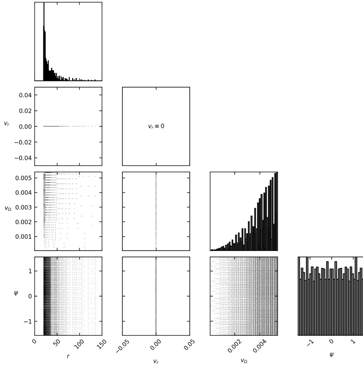
Figure 1. from Thomas R. Ruch et al 2026 Planet. Sci. J. 7 doi:10.3847/PSJ/aea3f4 https://dx.doi.org/10.3847/PSJ/aea3f4 © 2026. The Author(s). Published by the American Astronomical Society.
