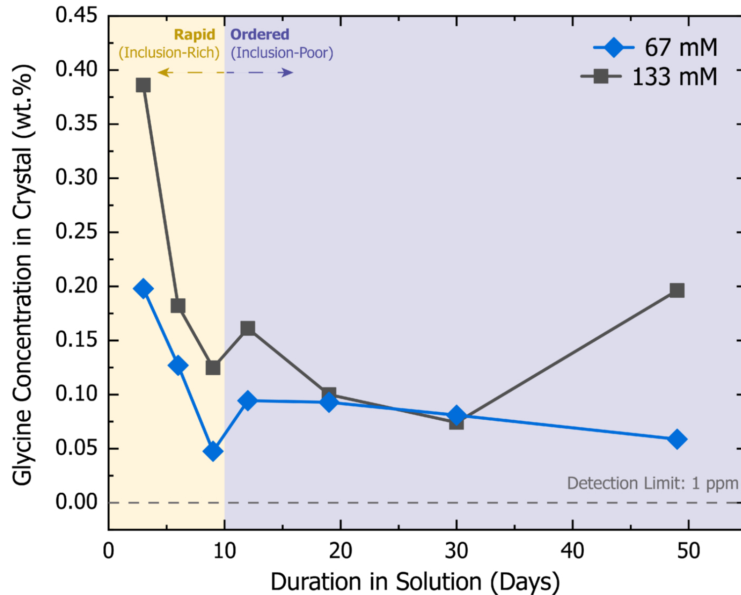
Figure 5. from Lucas R. Reynoso et al 2026 Planet. Sci. J. 7 doi:10.3847/PSJ/aea204 https://dx.doi.org/10.3847/PSJ/aea204 © 2026. The Author(s). Published by the American Astronomical Society.
