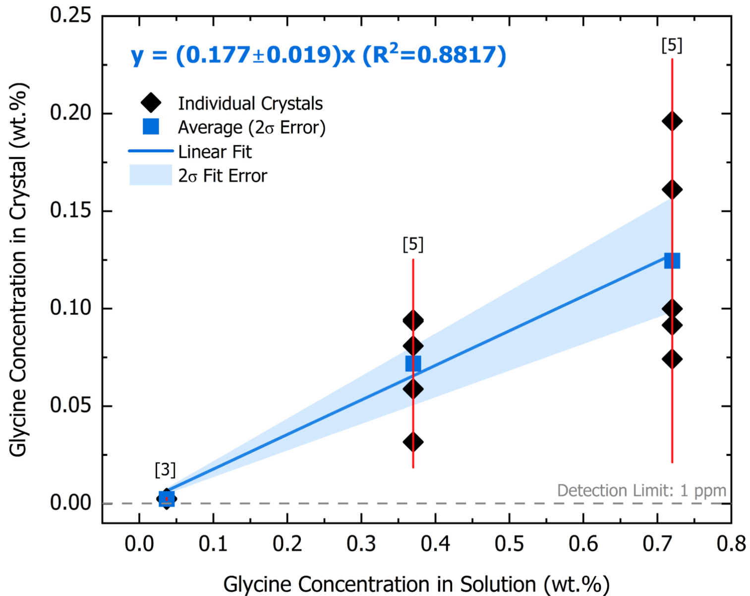
Figure 4. from Lucas R. Reynoso et al 2026 Planet. Sci. J. 7 doi:10.3847/PSJ/aea204 https://dx.doi.org/10.3847/PSJ/aea204 © 2026. The Author(s). Published by the American Astronomical Society.
