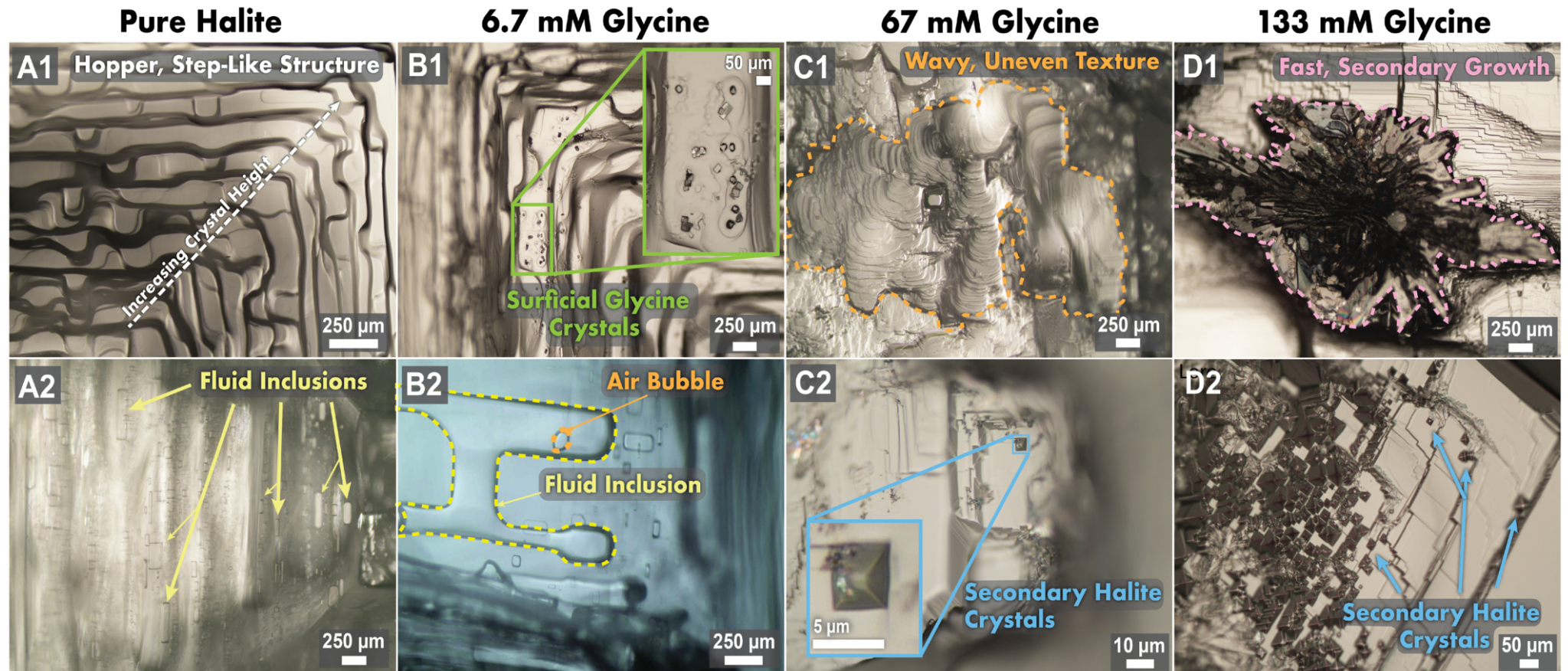
Figure 1. from Lucas R. Reynoso et al 2026 Planet. Sci. J. 7 doi:10.3847/PSJ/aea204 https://dx.doi.org/10.3847/PSJ/aea204 © 2026. The Author(s). Published by the American Astronomical Society.
