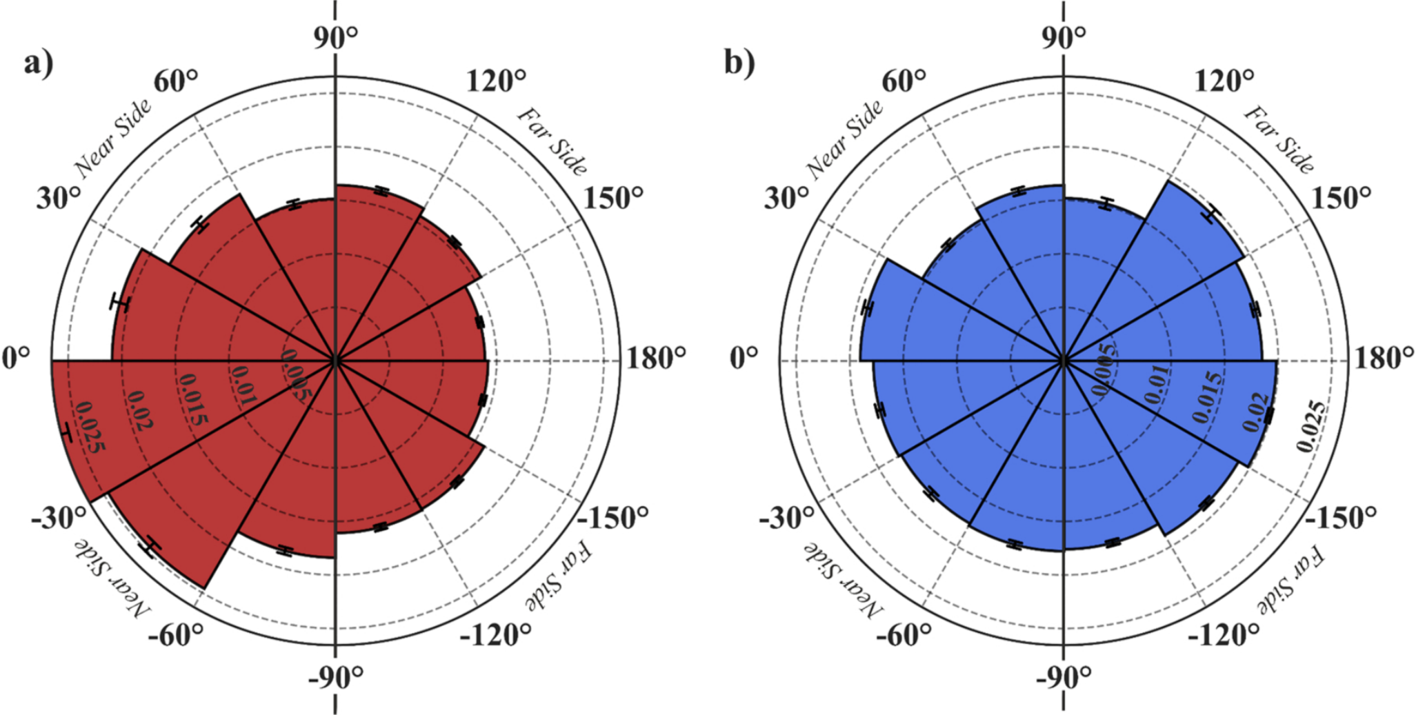
Figure 9. from Sachana Sathyan et al 2026 Planet. Sci. J. 7 doi:10.3847/PSJ/aea15c https://dx.doi.org/10.3847/PSJ/aea15c © 2026. The Author(s). Published by the American Astronomical Society.
