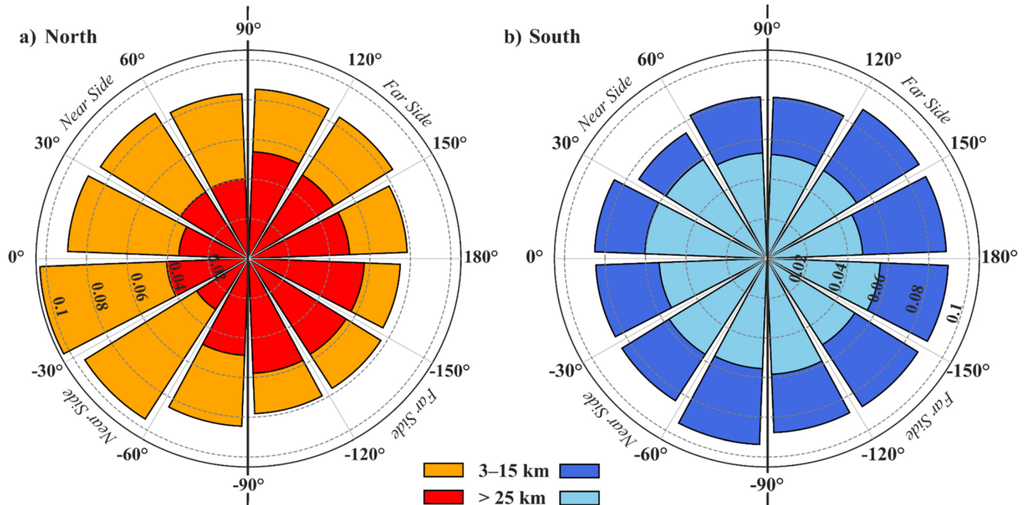
Figure 6. from Sachana Sathyan et al 2026 Planet. Sci. J. 7 doi:10.3847/PSJ/aea15c https://dx.doi.org/10.3847/PSJ/aea15c © 2026. The Author(s). Published by the American Astronomical Society.
