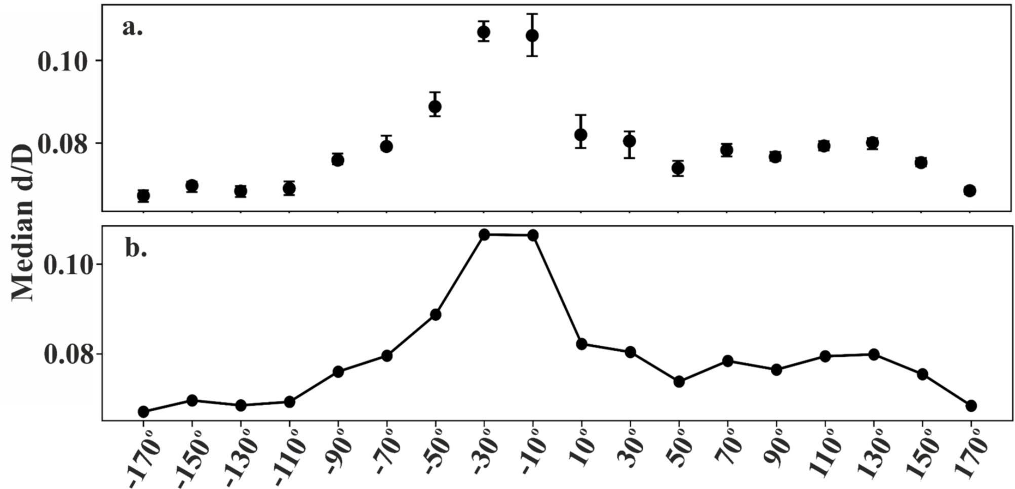
Figure B1. from Sachana Sathyan et al 2026 Planet. Sci. J. 7 doi:10.3847/PSJ/aea15c https://dx.doi.org/10.3847/PSJ/aea15c © 2026. The Author(s). Published by the American Astronomical Society.
