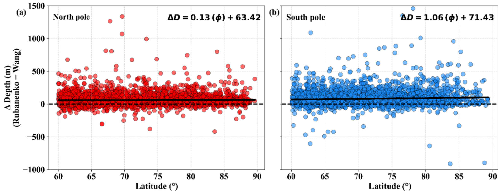
Figure A2. from Sachana Sathyan et al 2026 Planet. Sci. J. 7 doi:10.3847/PSJ/aea15c https://dx.doi.org/10.3847/PSJ/aea15c © 2026. The Author(s). Published by the American Astronomical Society.
