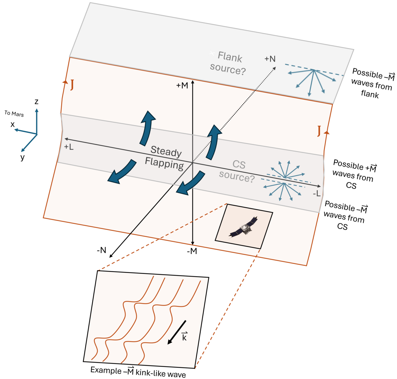
Figure 8. from Kyle Webster et al 2026 Planet. Sci. J. 7 doi:10.3847/PSJ/aea140 https://dx.doi.org/10.3847/PSJ/aea140 © 2026. The Author(s). Published by the American Astronomical Society.
