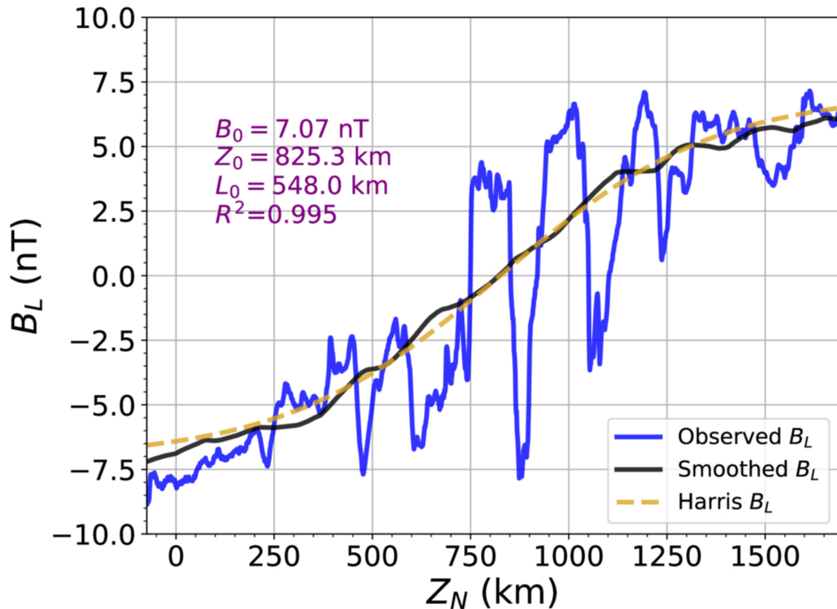
Figure 4. from Kyle Webster et al 2026 Planet. Sci. J. 7 doi:10.3847/PSJ/aea140 https://dx.doi.org/10.3847/PSJ/aea140 © 2026. The Author(s). Published by the American Astronomical Society.
