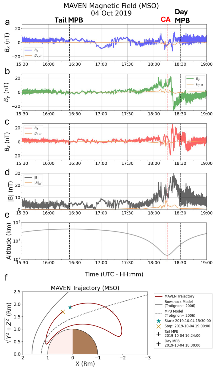
Figure 2. from Kyle Webster et al 2026 Planet. Sci. J. 7 doi:10.3847/PSJ/aea140 https://dx.doi.org/10.3847/PSJ/aea140 © 2026. The Author(s). Published by the American Astronomical Society.
