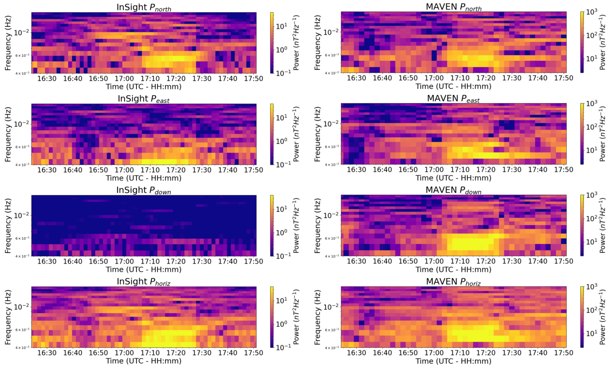
Figure 10. from Kyle Webster et al 2026 Planet. Sci. J. 7 doi:10.3847/PSJ/aea140 https://dx.doi.org/10.3847/PSJ/aea140 © 2026. The Author(s). Published by the American Astronomical Society.
