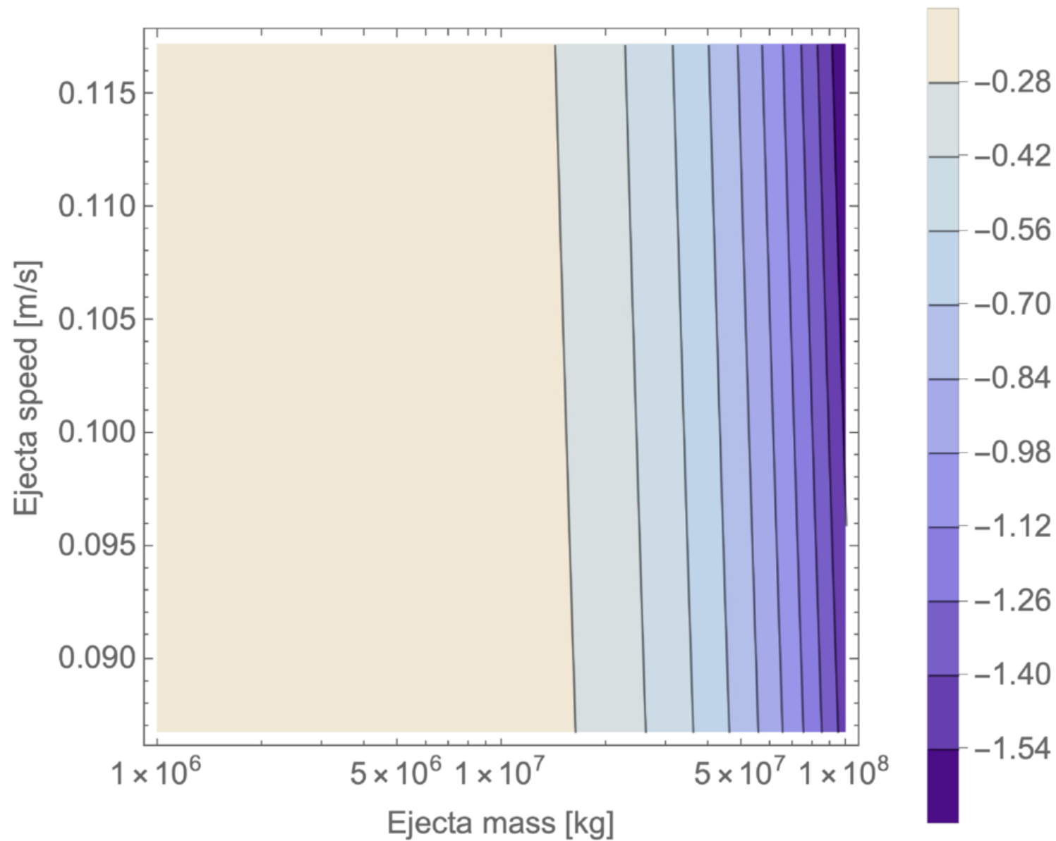
Figure 6. from Masatoshi Hirabayashi et al 2026 Planet. Sci. J. 7 doi:10.3847/PSJ/aea089 https://dx.doi.org/10.3847/PSJ/aea089 © 2026. The Author(s). Published by the American Astronomical Society.
