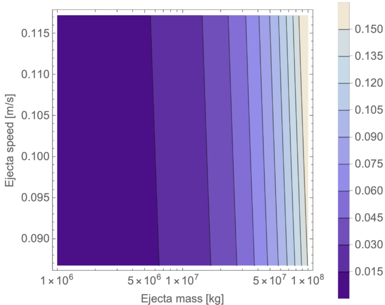
Figure 4. from Masatoshi Hirabayashi et al 2026 Planet. Sci. J. 7 doi:10.3847/PSJ/aea089 https://dx.doi.org/10.3847/PSJ/aea089 © 2026. The Author(s). Published by the American Astronomical Society.
