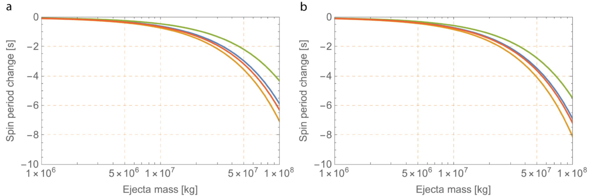
Figure 3. from Masatoshi Hirabayashi et al 2026 Planet. Sci. J. 7 doi:10.3847/PSJ/aea089 https://dx.doi.org/10.3847/PSJ/aea089 © 2026. The Author(s). Published by the American Astronomical Society.
