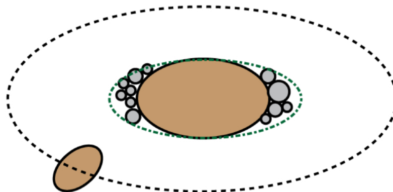
Accelerated spin due to ejecta accumulation
