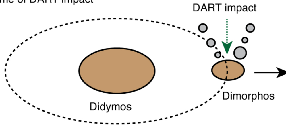
a. Time of DART impact
