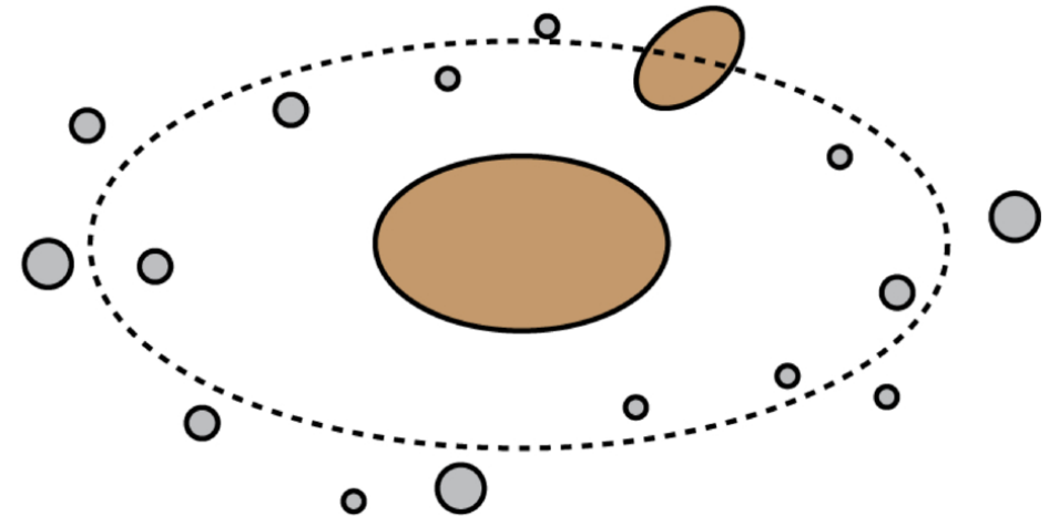
b. Initial orbit period change
