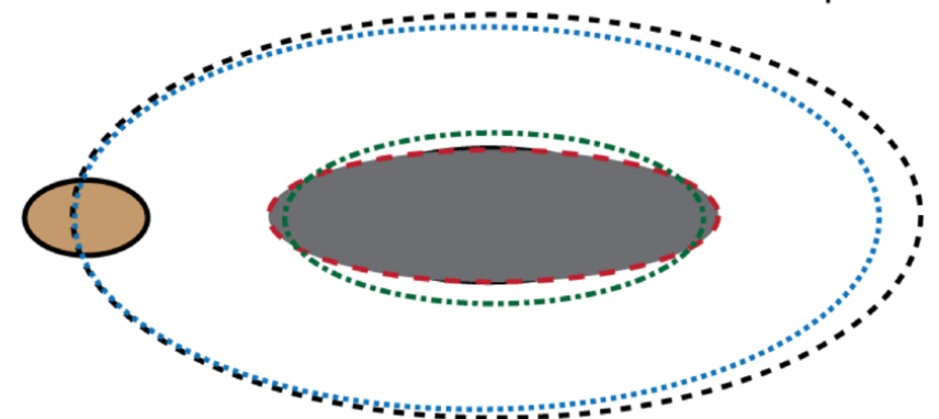
Spin-driven reshaping
