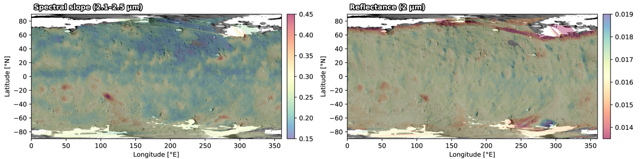
Figure 8. from Antonin Wargnier et al 2026 Planet. Sci. J. 7 doi:10.3847/PSJ/ae9fe7 https://dx.doi.org/10.3847/PSJ/ae9fe7 © 2026. The Author(s). Published by the American Astronomical Society.
