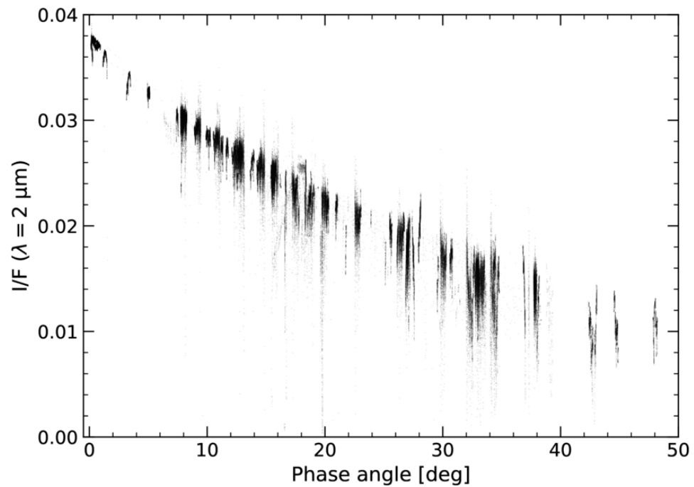
Figure 6. from Antonin Wargnier et al 2026 Planet. Sci. J. 7 doi:10.3847/PSJ/ae9fe7 https://dx.doi.org/10.3847/PSJ/ae9fe7 © 2026. The Author(s). Published by the American Astronomical Society.
