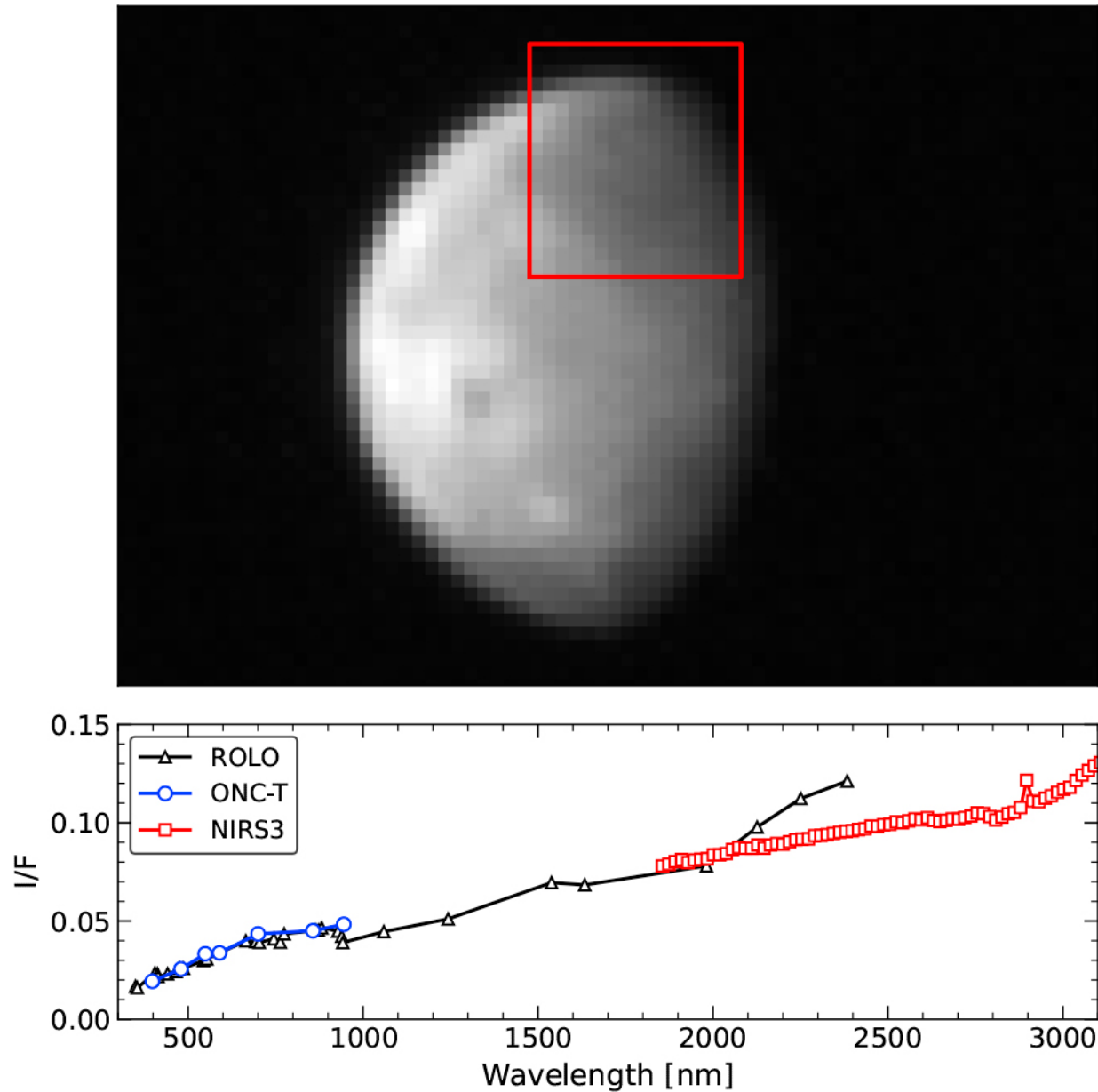
Figure 5. from Antonin Wargnier et al 2026 Planet. Sci. J. 7 doi:10.3847/PSJ/ae9fe7 https://dx.doi.org/10.3847/PSJ/ae9fe7 © 2026. The Author(s). Published by the American Astronomical Society.
