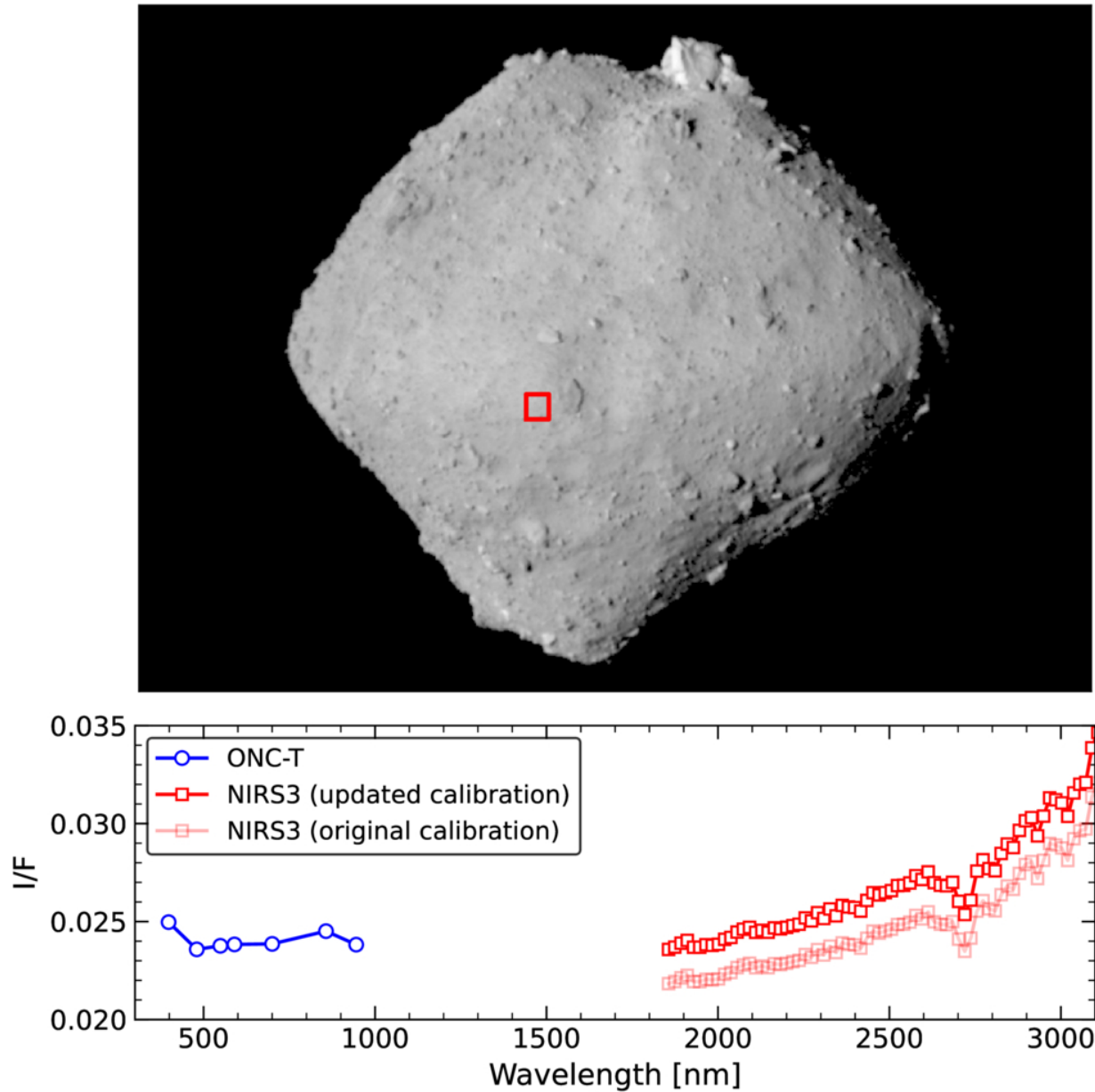
Figure 4. from Antonin Wargnier et al 2026 Planet. Sci. J. 7 doi:10.3847/PSJ/ae9fe7 https://dx.doi.org/10.3847/PSJ/ae9fe7 © 2026. The Author(s). Published by the American Astronomical Society.
