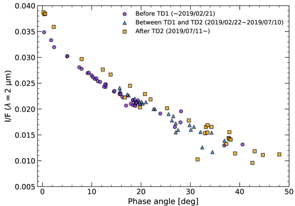
Figure 3. from Antonin Wargnier et al 2026 Planet. Sci. J. 7 doi:10.3847/PSJ/ae9fe7 https://dx.doi.org/10.3847/PSJ/ae9fe7 © 2026. The Author(s). Published by the American Astronomical Society.
