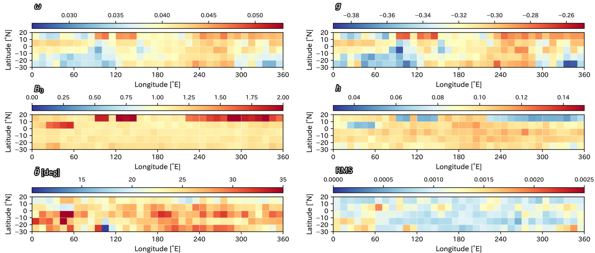
Figure J1. from Antonin Wargnier et al 2026 Planet. Sci. J. 7 doi:10.3847/PSJ/ae9fe7 https://dx.doi.org/10.3847/PSJ/ae9fe7 © 2026. The Author(s). Published by the American Astronomical Society.
