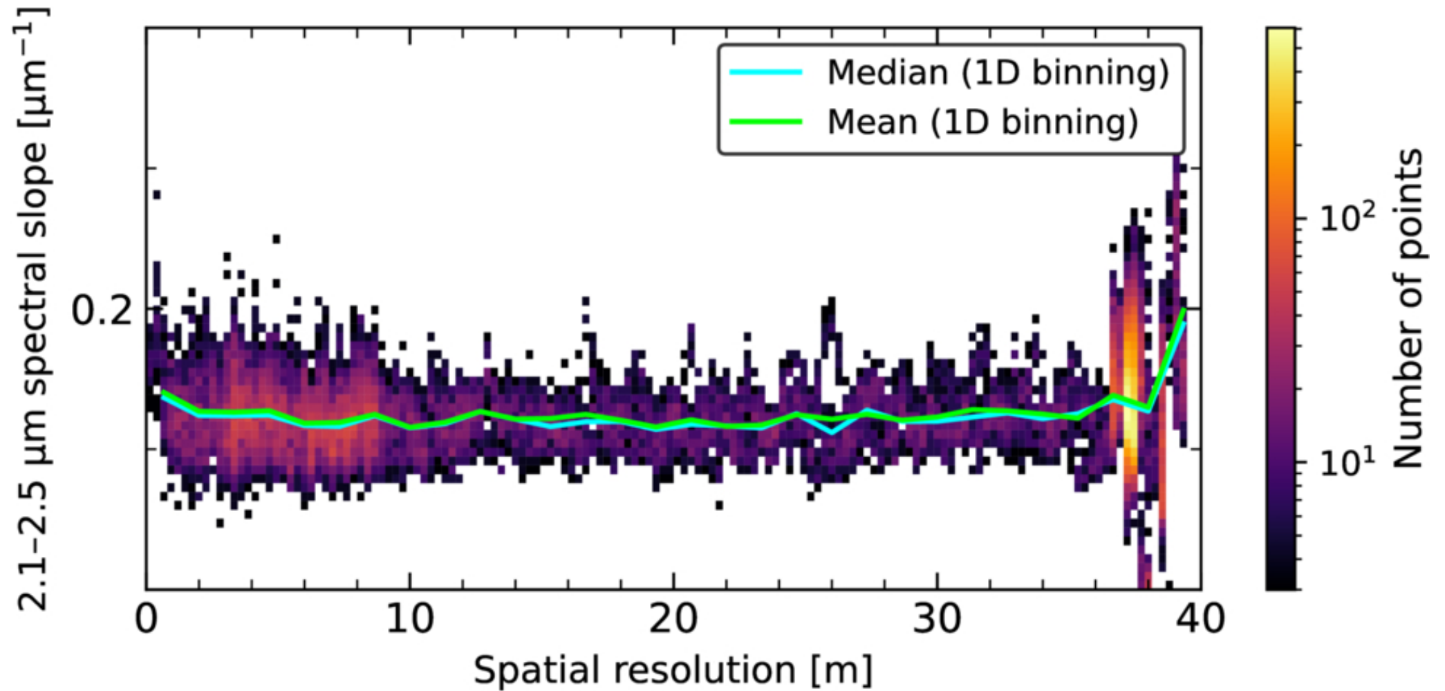
Figure I1. from Antonin Wargnier et al 2026 Planet. Sci. J. 7 doi:10.3847/PSJ/ae9fe7 https://dx.doi.org/10.3847/PSJ/ae9fe7 © 2026. The Author(s). Published by the American Astronomical Society.
