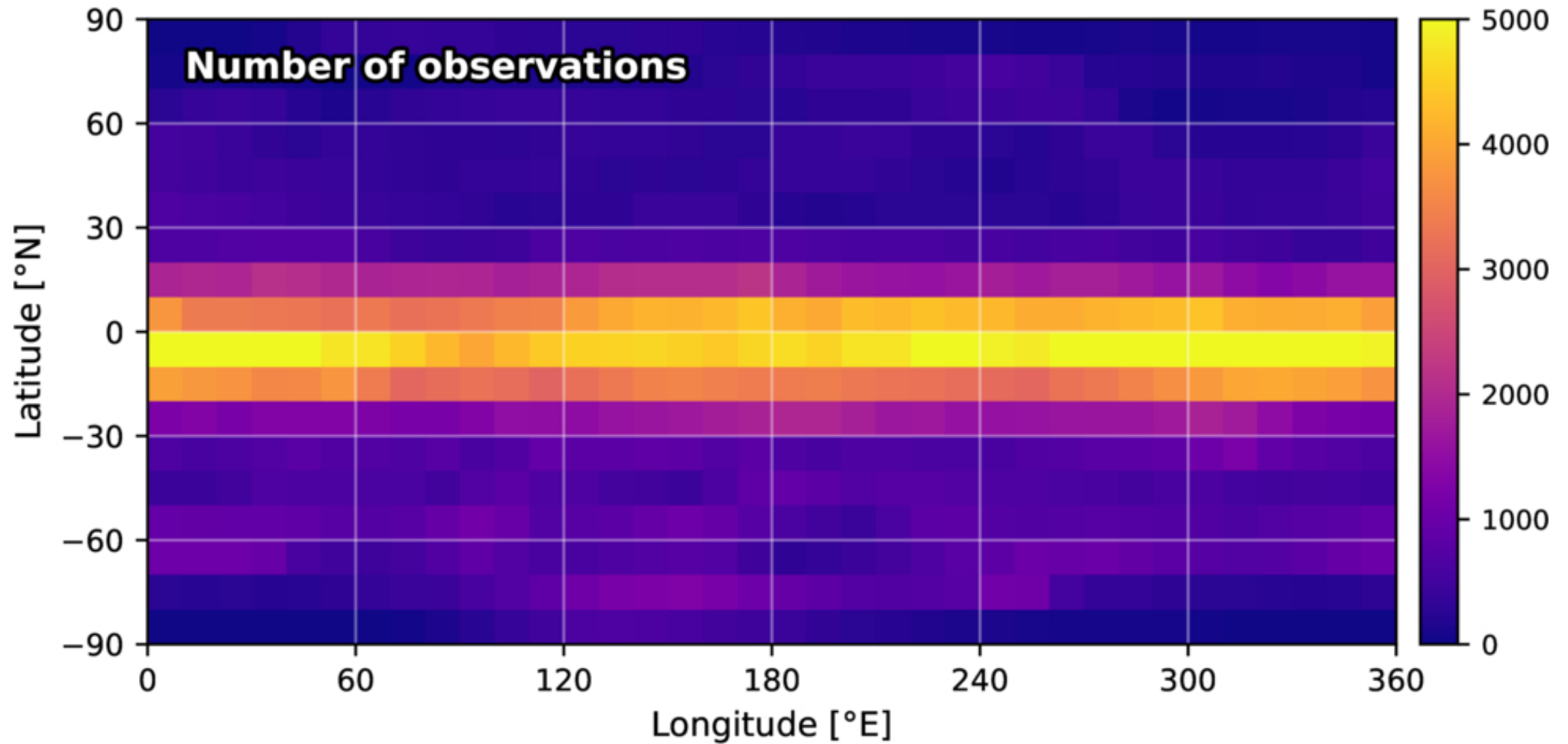
Figure F2. from Antonin Wargnier et al 2026 Planet. Sci. J. 7 doi:10.3847/PSJ/ae9fe7 https://dx.doi.org/10.3847/PSJ/ae9fe7 © 2026. The Author(s). Published by the American Astronomical Society.
