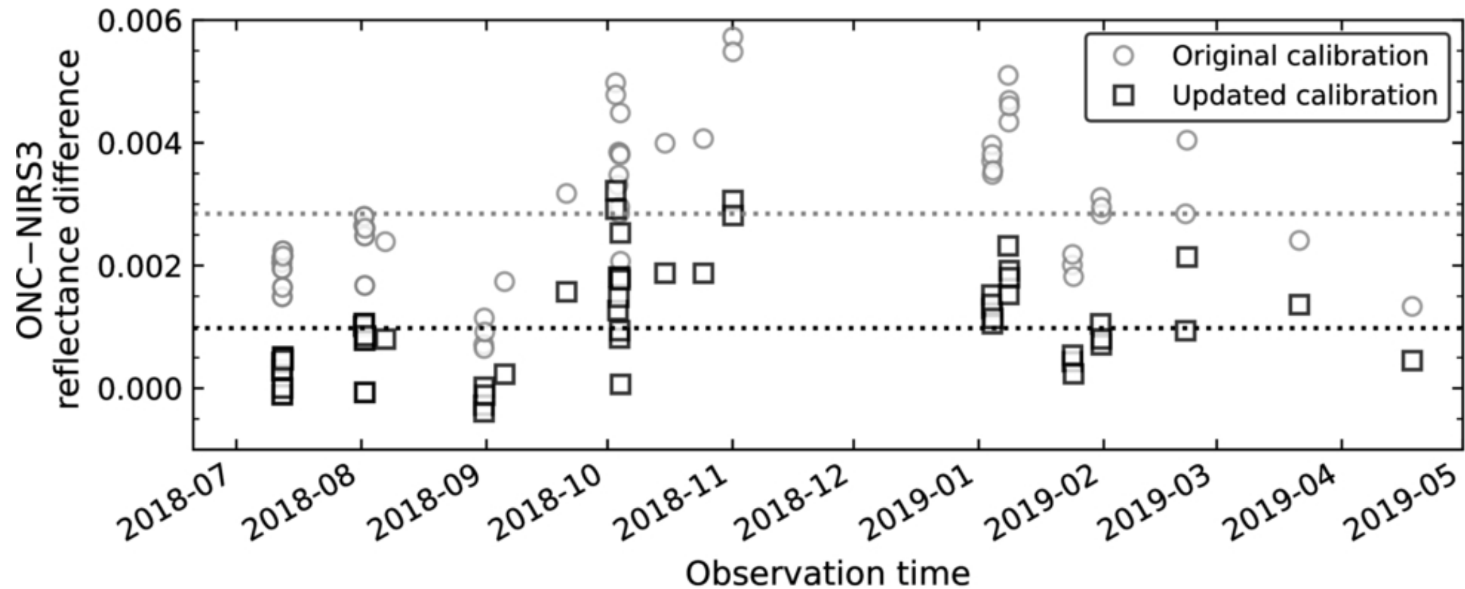
Figure E1. from Antonin Wargnier et al 2026 Planet. Sci. J. 7 doi:10.3847/PSJ/ae9fe7 https://dx.doi.org/10.3847/PSJ/ae9fe7 © 2026. The Author(s). Published by the American Astronomical Society.
