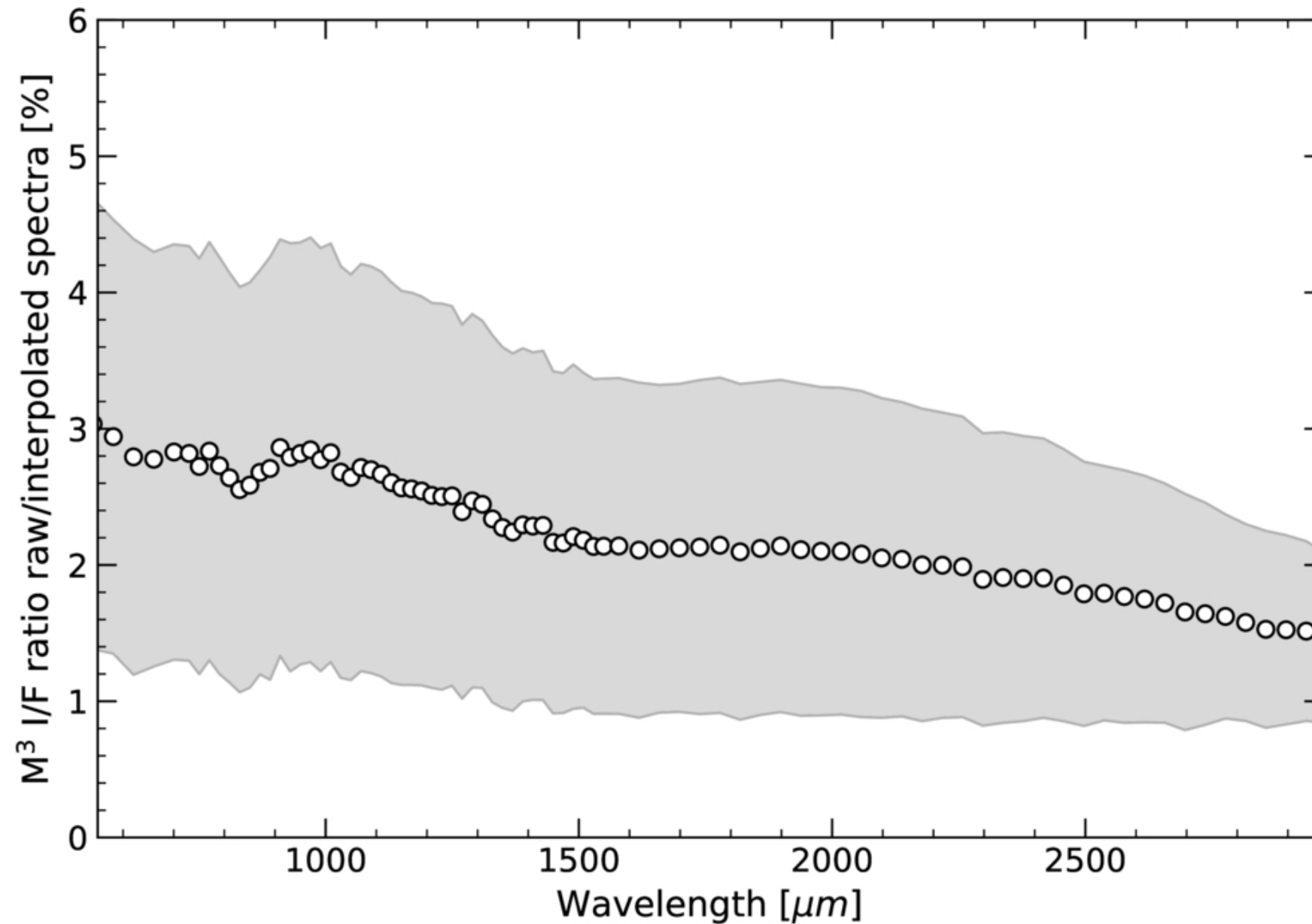
Figure C1. from Antonin Wargnier et al 2026 Planet. Sci. J. 7 doi:10.3847/PSJ/ae9fe7 https://dx.doi.org/10.3847/PSJ/ae9fe7 © 2026. The Author(s). Published by the American Astronomical Society.
