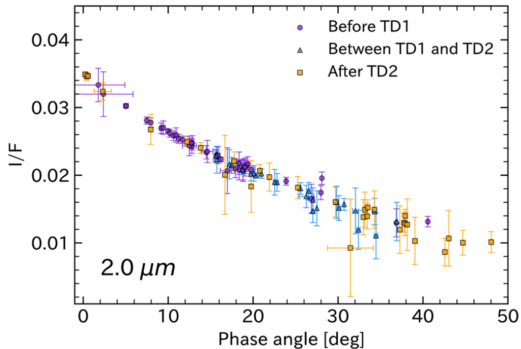
Figure A2. from Antonin Wargnier et al 2026 Planet. Sci. J. 7 doi:10.3847/PSJ/ae9fe7 https://dx.doi.org/10.3847/PSJ/ae9fe7 © 2026. The Author(s). Published by the American Astronomical Society.
