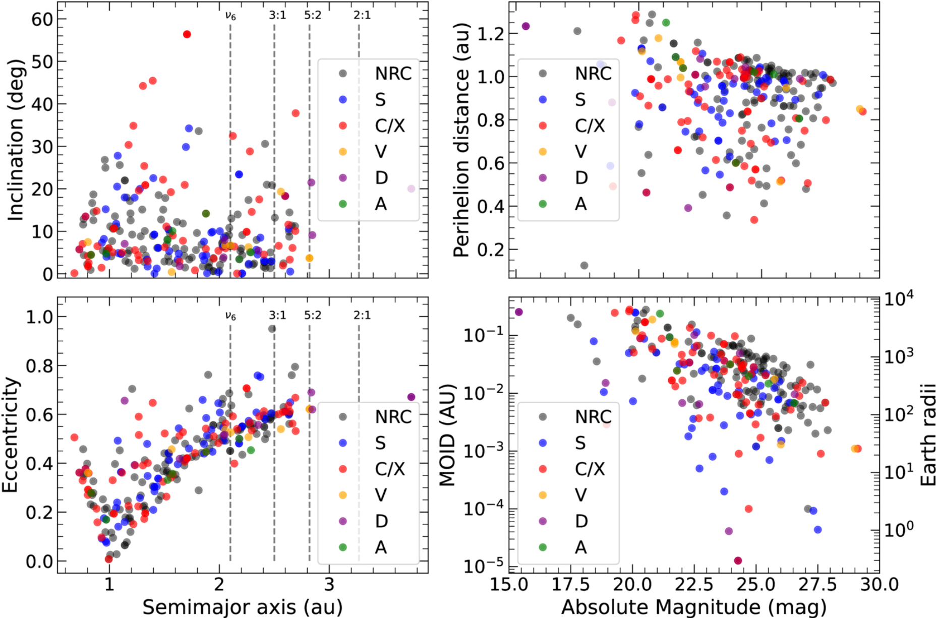
Figure 8. from Andy J. López-Oquendo et al 2026 Planet. Sci. J. 7 doi:10.3847/PSJ/ae9f3f https://dx.doi.org/10.3847/PSJ/ae9f3f © 2026. The Author(s). Published by the American Astronomical Society.
