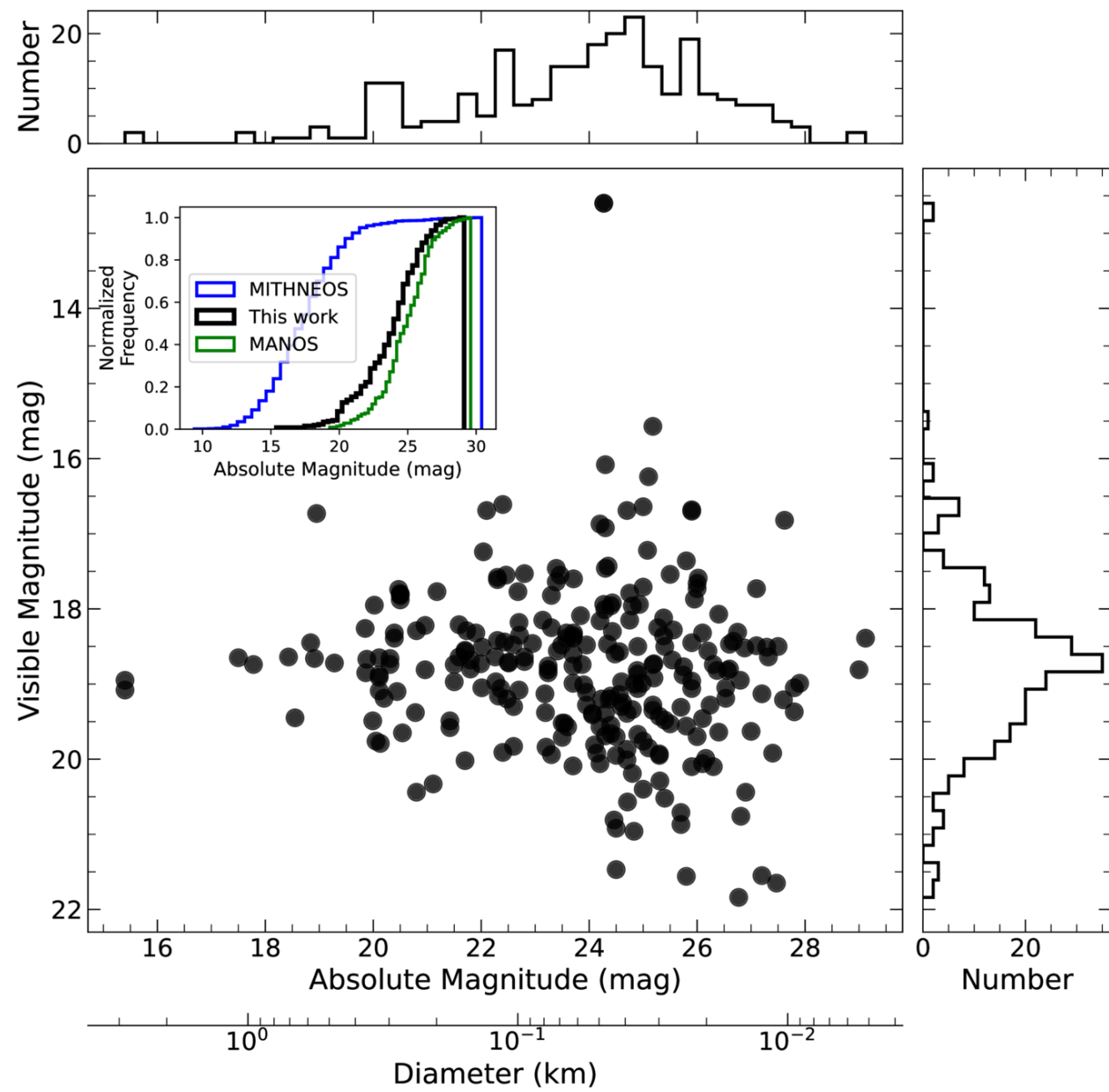
Figure 5. from Andy J. López-Oquendo et al 2026 Planet. Sci. J. 7 doi:10.3847/PSJ/ae9f3f https://dx.doi.org/10.3847/PSJ/ae9f3f © 2026. The Author(s). Published by the American Astronomical Society.
