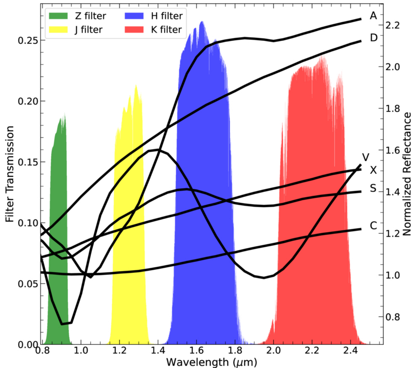
Figure 2. from Andy J. López-Oquendo et al 2026 Planet. Sci. J. 7 doi:10.3847/PSJ/ae9f3f https://dx.doi.org/10.3847/PSJ/ae9f3f © 2026. The Author(s). Published by the American Astronomical Society.
